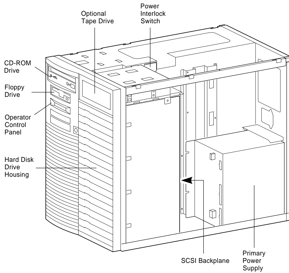
Figure 5 AlphaServer 1000 System Front View
