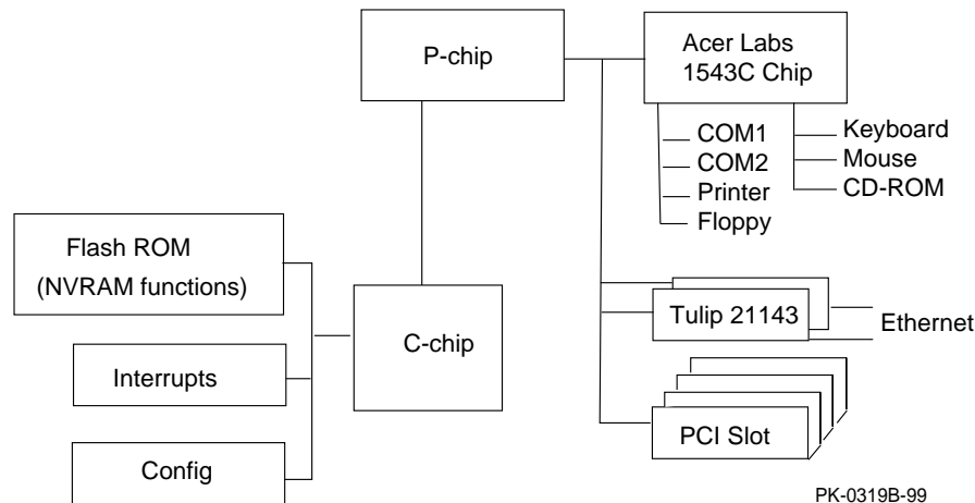
Block Diagram of I/O Control
