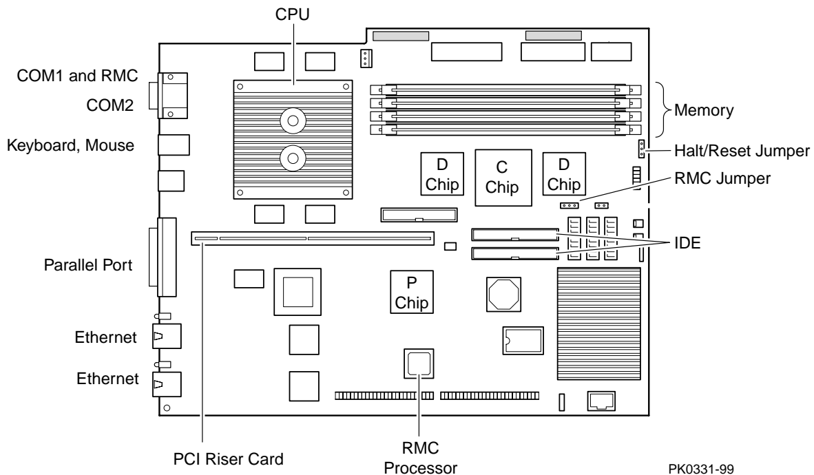
Component and Connector Locations
