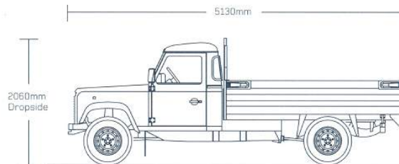
WHEEL BASE 130 SINGLE CAB
