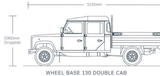
WHEEL BASE 130 DOUBLE CAB
