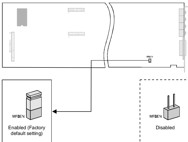
Figure C-1: The available MPU-401 MIDI Emulation settings.
