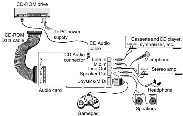
Figure 1-4: Connecting external speakers and other devices.
