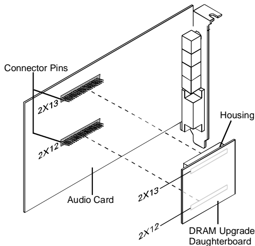
Figure 1-2: Mounting the DRAM Upgrade daughterboard.
