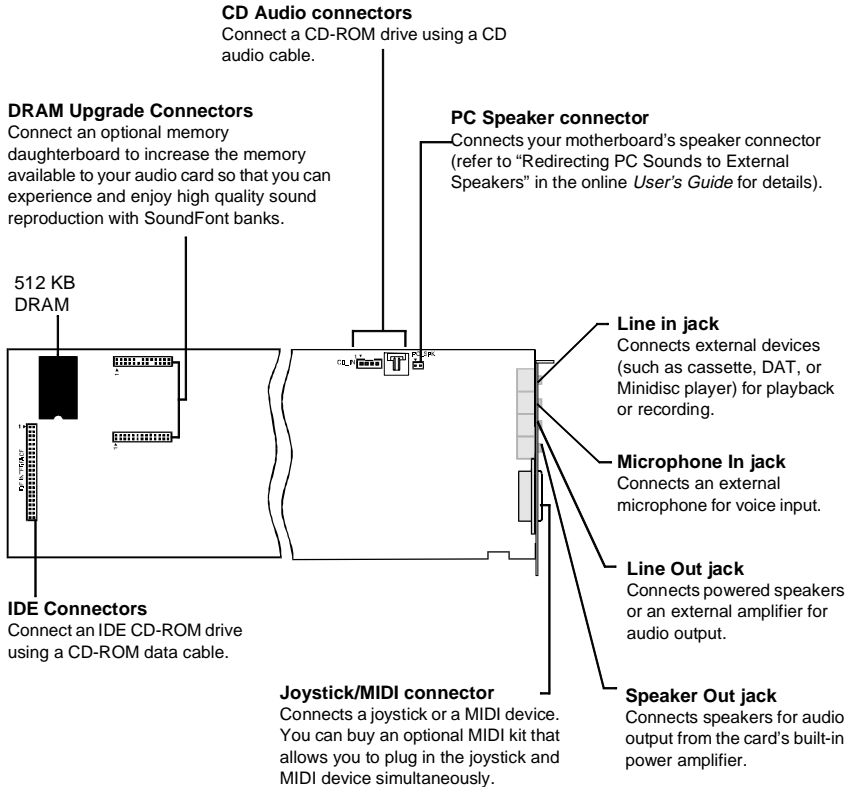
Figure 1-1: The connectors on your audio card.
